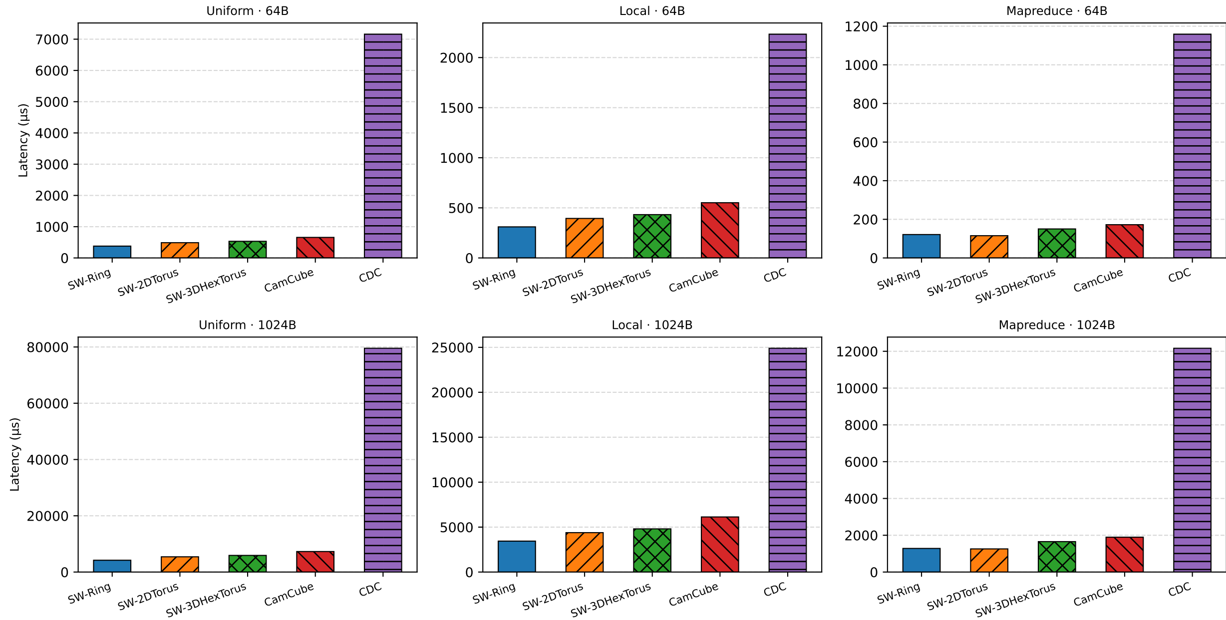
Fig. 5 — Packet Delivery Latency (N=512)
